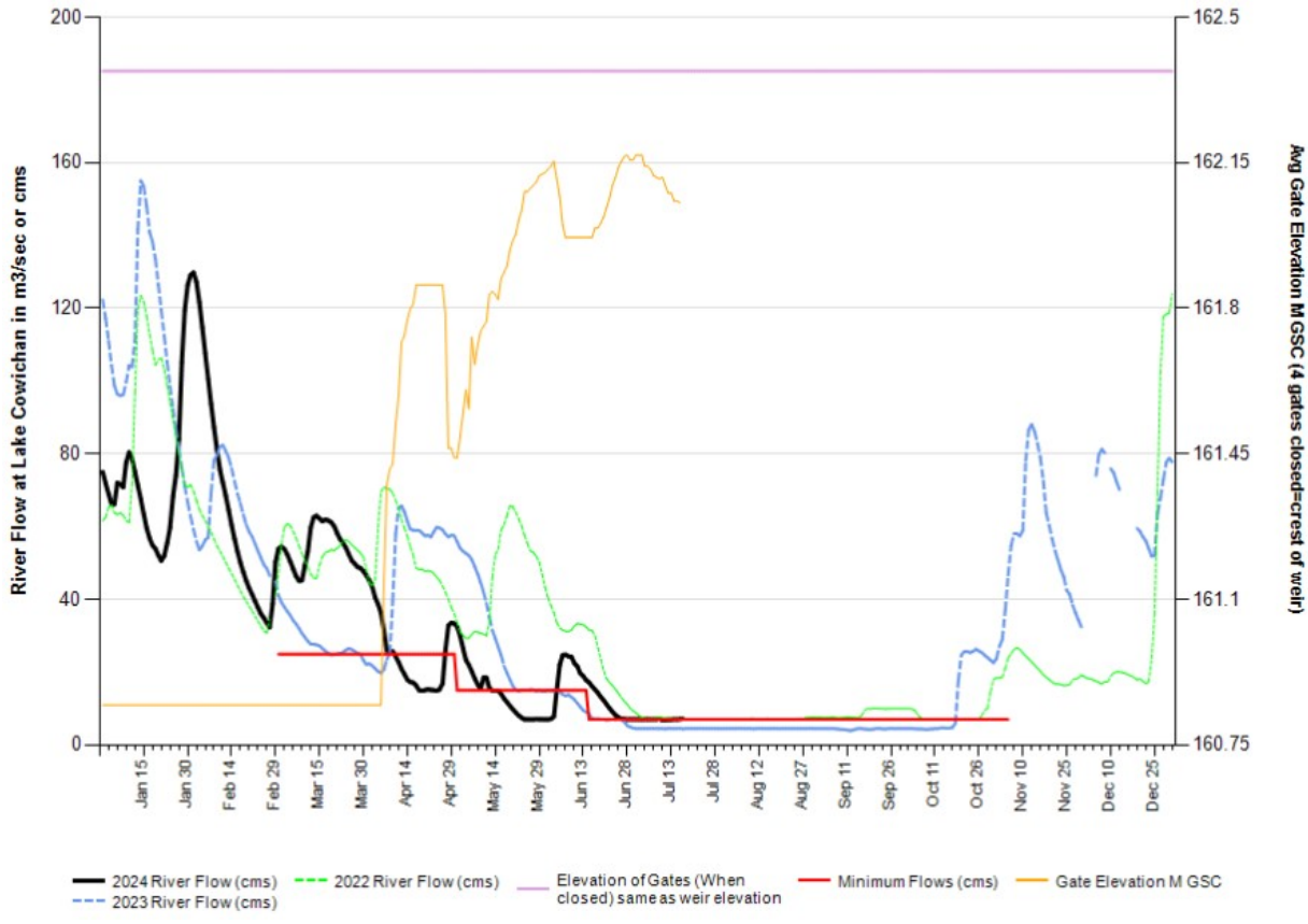
2024 Cowichan River Flow - 2024 (Black) & 2023 (Blue) & 2022 (Green)
