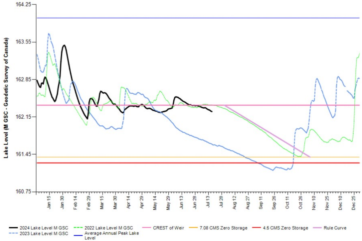
2024 Cowichan Lake Level - 2024 (Black) & 2023 (Blue) & 2022 (Green)
