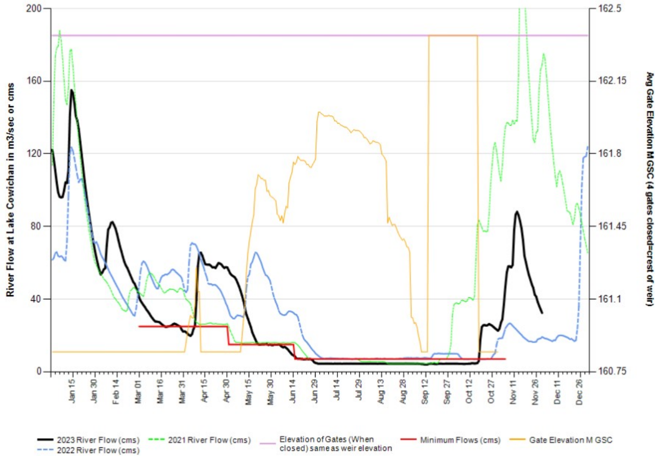
2023 Cowichan River Flow - 2023 (Black) & 2022 (Blue) & 2021 (Green)
